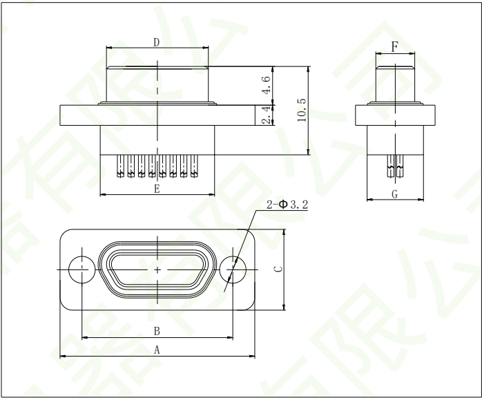
J30JY-□TJ
